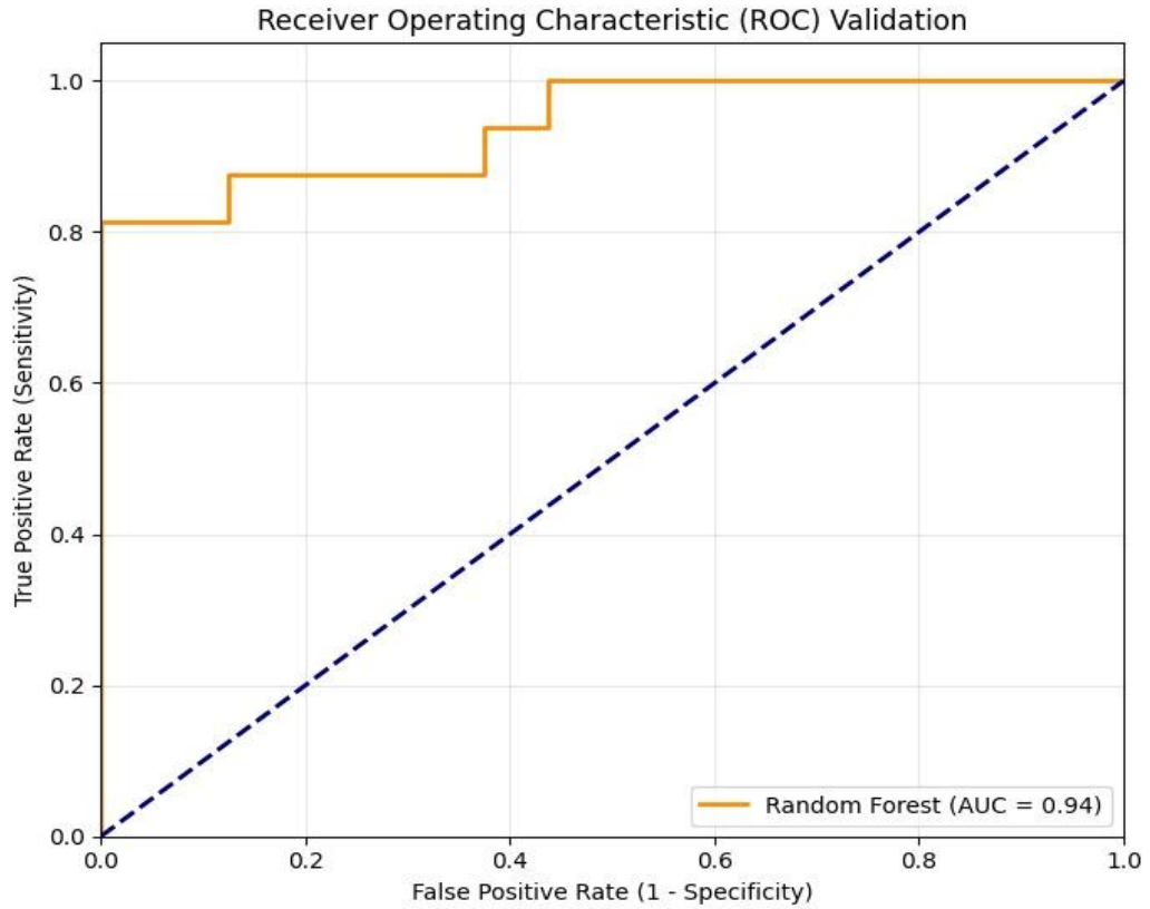
Figure 3: ROC-AUC Validation Curve of the Random Forest Model (AUC = 0.94), Gilgit District
