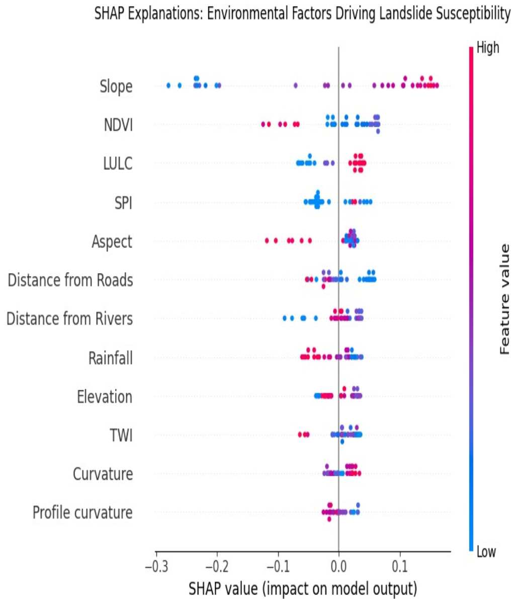
Figure 6: SHAP Summary Plot
