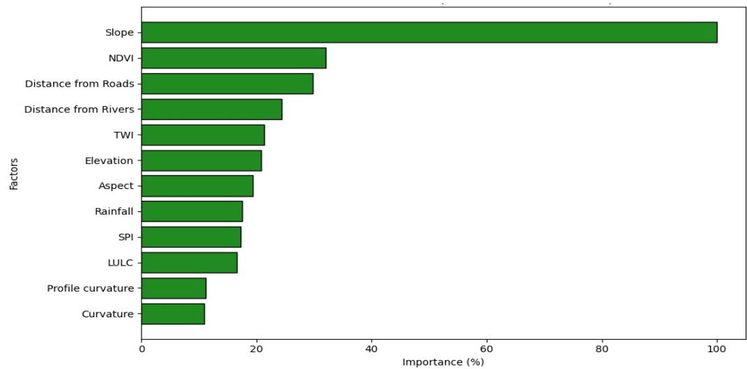
Figure 5: Random Forest Feature Importance
